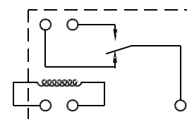
接线图 (底视图) Wiring Diagram (Bottom View)
